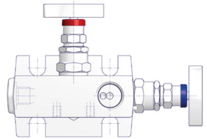
T-Style 2 Valve Manifolds C13ST-2T[ ]A2 Type Isolate Valve optional on right side
