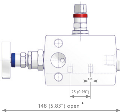
H-Style 2 Valve Manifolds C13ST-2H[ ]B1 Type Flanged x Flanged
