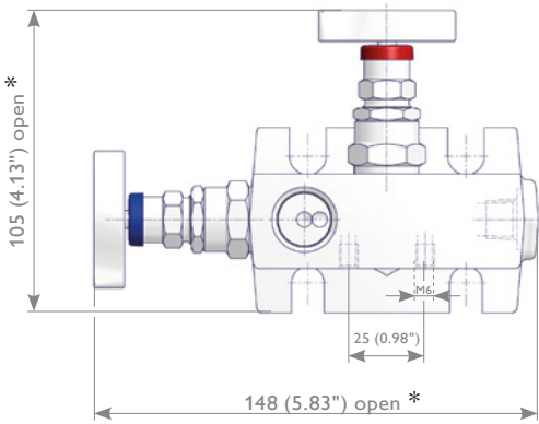
T-Style 2 Valve Manifolds C13ST-2T[ ]A1 Type 1/2 NPT Female x Flanged
