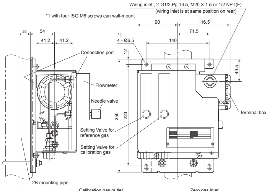
2B pipe mounting example
